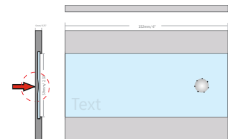
Option D : with Dimple to keep the insert
