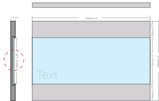
Option A : 2mm clear Acrylic 0.08"
